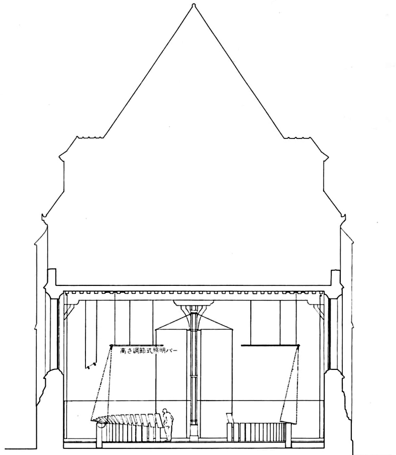
X-XSECTION 1:100
